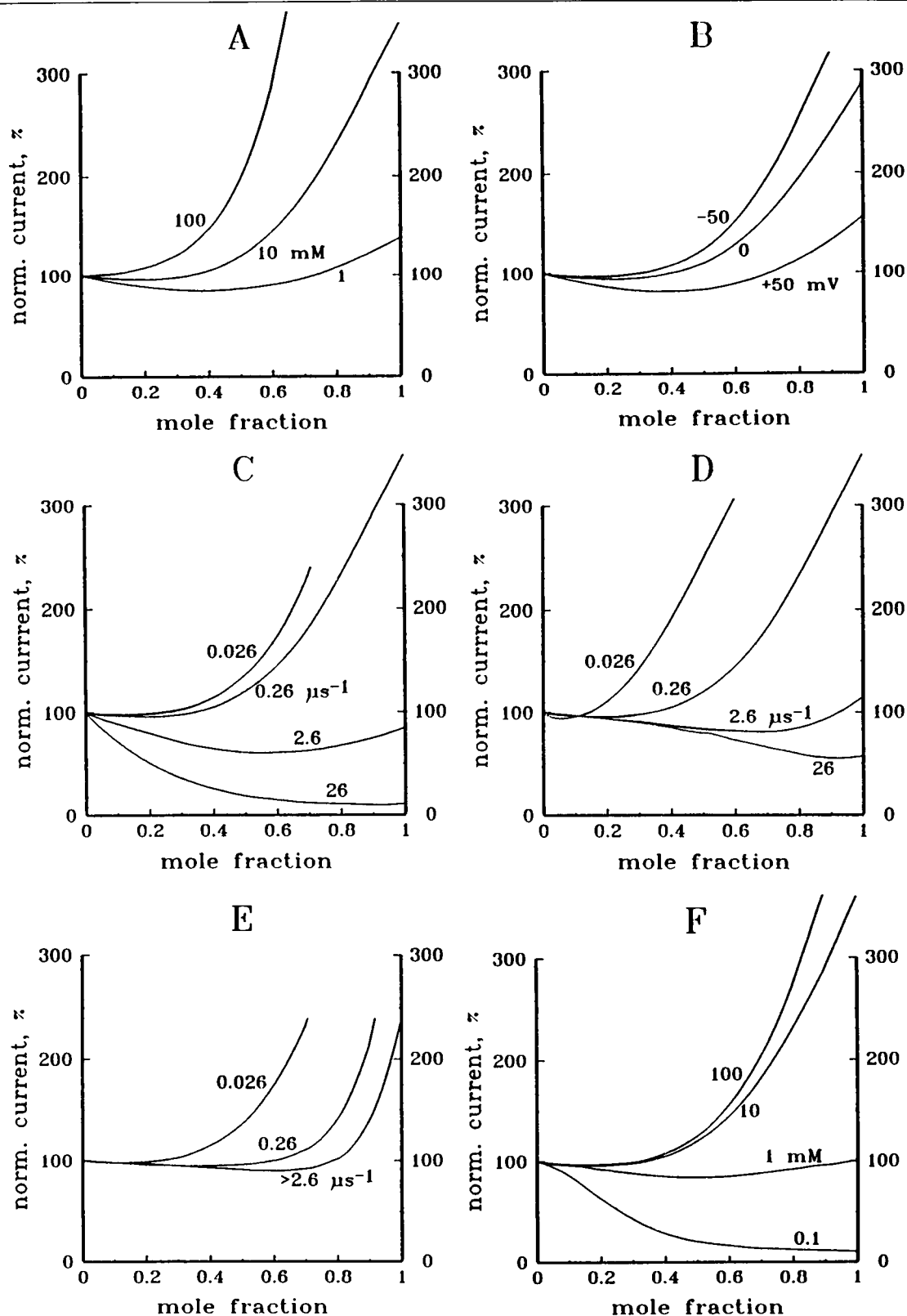
FIGURE 2 Anomalous mole fraction effect for the conformational model. Two permeant ions (Ca and Ba) were present only in the external compartment ( [Ca]_{in} = [Ba]_{in} = 0 ) and except in (A) their total concentration was 10 mM. The current calculated at -25 mV was normalized to the amplitude of pure calcium current and was plotted vs the mole fraction of Ba. All the calculations were made with the basic set of parameters for Ca and Ba listed in the Theory section with variations of total concentration of divalent cations (A), membrane voltage (B), rate constant for the first conformational transition c (C), rate constant for the second conformational transition d (D), dissociation constant for the low-affinity site for Ba (F). In (E) both rate constants for conformational transitions were varied with c = d . Corresponding numerical values of model parameters are indicated near each curve.
