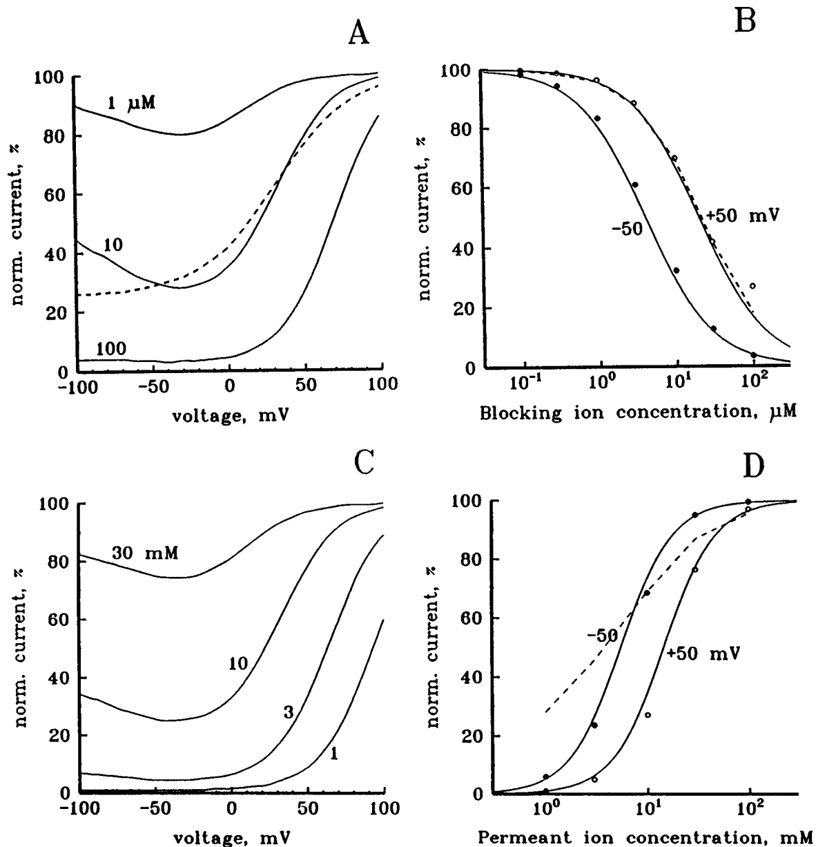
FIGURE 3 The external ion block for the conformational model in symmetrical conditions. All the calculations were made with the basic set of parameters listed in the Theory section for Ca as a permeable ion. For blocking ion X all parameters were the same except the dissociation constants for the high-affinity binding site K'_X = 0.01 \mu\text{M} and the rate constant for the first conformational transition c_X = 0 . [X]_{\text{in}} = 0 . (A) Voltage dependence of block calculated for different concentrations of the blocking ion indicated near each curve. C_{\text{in}} = C_{\text{out}} = 10 \text{ mM} . Superimposed is a dotted curve showing the block for the 2BIS model calculated for [X]_{\text{out}} = 10 \mu\text{M} with K_{\text{Ca}} = 1 \text{ mM} and K_X = 0.3 \mu\text{M} . (B) Circles show the concentration dependence of block for two voltages (as indicated near each curve) plotted from the results of calculations exemplified in (A). Smooth curves were drawn according to a Michaelis-Menten type equation I_{\text{norm}} = K_X[X]/(K_X + [X]) with apparent dissociation constant K_X of 4 \mu\text{M} at -50 \text{ mV} and 20 \mu\text{M} at +50 \text{ mV} . A dotted line calculated at +50 \text{ mV} using the 2BIS model with parameters listed in A. (C) Voltage dependence of block calculated for different concentration of the permeant ions ( C_{\text{in}} = C_{\text{out}} ) indicated near each curve. [X]_{\text{out}} = 10 \mu\text{M} . (D) Circles show the concentration dependence of block for two voltages (as indicated near each curve) plotted from the results of calculations exemplified in C. Smooth curves were drawn according to the Hill equation I_{\text{norm}} = ([\text{Ca}]/(K_{\text{Ca}} + [\text{Ca}]))^n with n = 1.7 and the apparent dissociation constant K_{\text{Ca}} = 3 \mu\text{M} at -50 \text{ mV} and 15 \mu\text{M} at +50 \text{ mV} . Dotted curve calculated at +50 \text{ mV} using the 2BIS model with parameters used in A.
