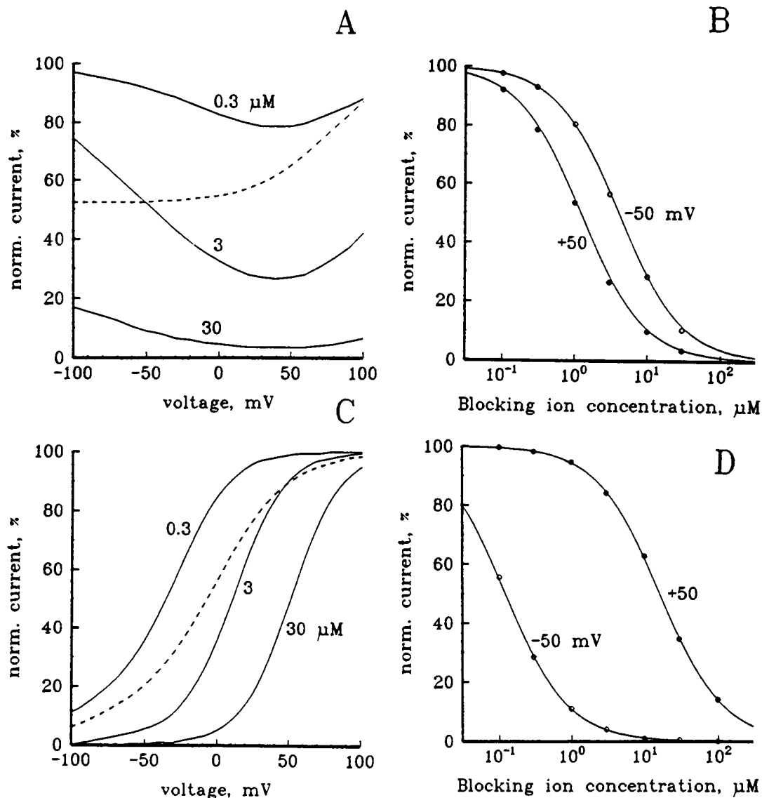
FIGURE 4 External ion block of unidirectional currents for the conformational model. All the calculations were made using the conformational model with parameters given in legend to Fig. 3. [X]_{in} = 0 , [C]_{in} = 0 for A and B, and [C]_{out} = 0 for C and D. (A) Voltage dependence of external ion block of the inward current calculated for different concentrations of the blocking ion ( X ) indicated near each curve. X_{out} = 10 \mu M , C_{out} = 10 \text{ mM} , C_{in} = 0 . Dotted curve shows the block for the 2B1S model calculated for [X]_{out} = 3 \mu M with K_{Ca} = 1 \text{ mM} and K_X = 0.3 \mu M . (B) Circles show the concentration dependence of block for two voltages (as indicated near each curve) plotted from the results of calculations exemplified in A. Smooth curves were drawn according to a Michaelis-Menten type equation I_{norm.} = K_X[X]/(K_X + [X]) with the apparent dissociation constant K_X = 4 \mu M at +50 \text{ mV} and 1.2 \mu M at -50 \text{ mV} . (C) Voltage dependence of external ion block of the outward current calculated for different concentrations of the blocking ion indicated near each curve. X_{out} = 10 \mu M , C_{in} = 10 \text{ mM} , C_{out} = 0 . Dotted curve shows the block for the 2B1S model calculated with parameters listed in A. (D) Circles show the concentration dependence of block for two voltages (as indicated near each curve) plotted from the results of calculations exemplified in C. Smooth curves were drawn according to a Michaelis-Menten type equation I_{norm.} = K_X[X]/(K_X + [X]) with the apparent dissociation constant K_X = 0.12 \mu M at -50 \text{ mV} and 16 \mu M at +50 \text{ mV} .
