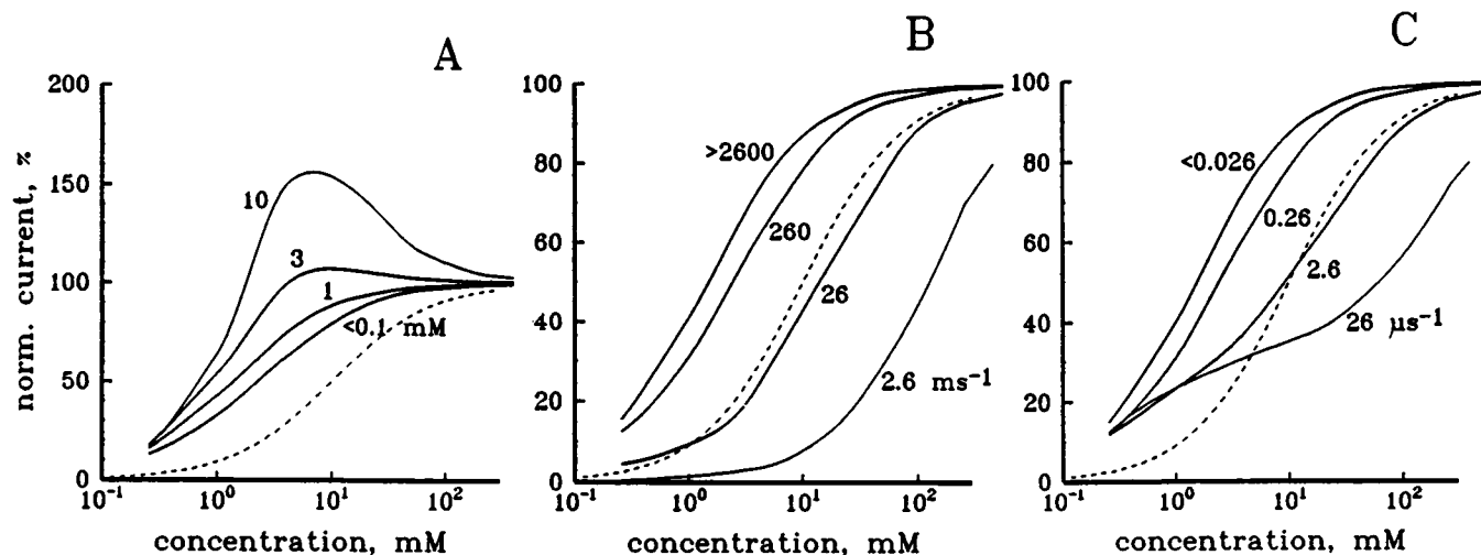
FIGURE 1 Concentration dependence of the channel current for the conformational model. All the calculations were made with the basic set of parameters for Ca listed in the Theory section with variations indicated near each curve. Calculated current at -25 mV was normalized to its limiting value at high concentrations. Permeant ions were present only in the external compartment ( [Ca]_{in} = 0 ) and their concentration was plotted on the abscissa. For each frame only a single parameter was varied: dissociation constant for the high-affinity binding site (A), rate constants for the first conformational transition (B), and for the second conformational transition (C), with the numerical values indicated near each curve. Dotted line in each frame shows the concentration dependence for the one-ion model (2B1S) with the dissociation constant of 10 mM.
