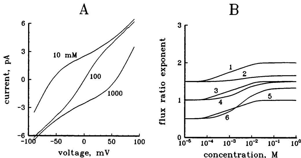
FIGURE 5 Ussing flux ratio for the conformational model. All the calculations were made with the basic set of parameters for Ca listed in the Theory section but the charge of permeant cation was set to +1. (A) Voltage dependence of the total channel current calculated with the basic set of model parameters. Electrical distances were chosen as follows: in the first conformational state all \sigma_i^+ = 0.25 , in the second conformational state \sigma_1^+ = \sigma_2^+ = 0.5 , \sigma_{-1}^+ = \sigma_{-2}^+ = 0 for an ion entering the channel from the external compartment, \sigma_1^- = \sigma_2^- = 0 , \sigma_{-1}^- = \sigma_{-2}^- = 0.5 for an ion entering the channel from the internal compartment. C_{out} = 100 mM and C_{in} is indicated near each curve. (B) Concentration dependence of the exponent in the Ussing flux ratio. Permeant ions were present in the external and the internal compartments in equal concentration plotted on abscissa. Calculations were made for the basic set of model parameters with the following modifications: dissociation constant in the first conformational state was 1 \mu M (curves 1, 3 and 5) and 1 mM (curve 2, 4 and 6); in the first conformational state all \sigma_i^+ = 0.25 , and in the second conformational state \sigma_1^+ = \sigma_2^+ = 0.5 , \sigma_{-1}^+ = \sigma_{-2}^+ = 0 , \sigma_1^- = \sigma_2^- = 0 , \sigma_{-1}^- = \sigma_{-2}^- = 0.5 (curves 1, 2); all \sigma_i^+ = \sigma_i^- = 0.25 (curves 3, 4); \sigma_1^+ = \sigma_2^+ = 0 , \sigma_{-1}^+ = \sigma_{-2}^+ = 0.5 , \sigma_1^- = \sigma_2^- = 0.5 , \sigma_{-1}^- = \sigma_{-2}^- = 0 (curves 5, 6).
